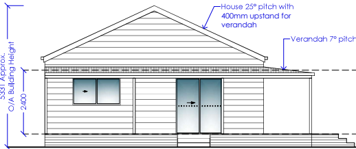
East Elevation
