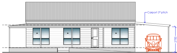
North Elevation
